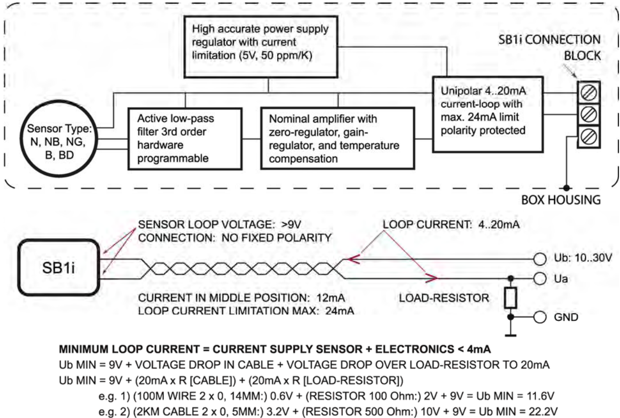
FIGURE 4: Block Diagram and Wiring Connections
