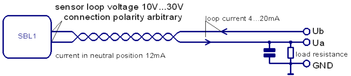
FIGURE 1: Cable Connections
